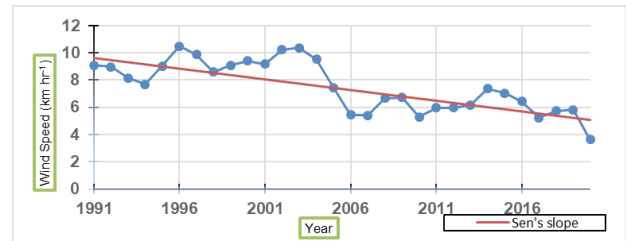
Fig. 9. Showing the trend and sen's slope of wind speed for Akola district. It indicates that Man-Kendall test has p- value less than level of significance. i.e. 0.05, so as per test statistics it is concluded that wind speed have trend in it's time series and sen's slope having neagtive value which indicates that there is decreasing trend over period of time.
