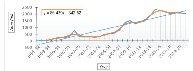
Fig. 1. Showing the time series analysis for the area (ha) under soybean in Akola district by using three years moving average method. From fig. it is clearly observed that area under soybean in Akola district is rising over period of time.
