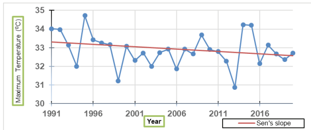
Fig. 5. Showing the trend and sen's slope of maximum temperature for Akola district. It indicates that Man-Kendall test has p- value greater than level of significance. i.e. 0.05, so as per test statistics it is concluded that maximum temperature for does not have trend in it's time series.
