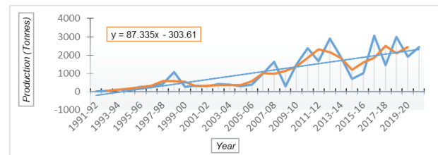
Fig. 2. Showing the time series analysis for the production (Tonnes) under soybean in Akola district by using three years moving average method. It is observed that productivity of soybean in Akola district is increasing over period of time.
