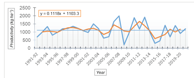
Fig. 3. Showing the time series analysis for the productivity (kg ha -1 ) under soybean in Akola district by using three years moving average method. From fig. it is clearly observed that productivity of soybean in Akola district is constant growing over period of time.
