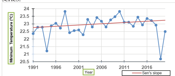
Fig. 6. Showing the trend and sen's slope of minimum temperature for Akola district. It indicates that Man-Kendall test has p- value greater than level of significance. i.e. 0.05, so as per test statistics it is concluded that minimum temperature for does not have trend in it's time series.
