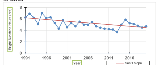
Fig. 10. Showing the trend and sen's slope of bright sunshine hours for Akola district. It indicates that Man-Kendall test has p- value less than level of significance. i.e. 0.05, so as per test statistics it is concluded that bright sunshine hours have trend in it's time series and sen's slope having neagtive value which indicates that there is decreasing trend over period of time.
