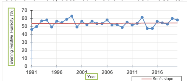
Fig. 8. Showing the trend and sen's slope of evening relative humidity for Akola district. It indicates that Man-Kendall test has p- value greater than level of significance. i.e. 0.05, so as per test statistics it is concluded that evening relative humidity does not have trend in it's time series.
