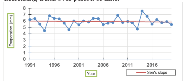
Fig. 11. Showing the trend and sen's slope of evaporation for Akola district. It indicates that Man-Kendall test has p- value less than level of significance. i.e. 0.05, so as per test statistics it is concluded that evaporation does not have trend in it's time series.
