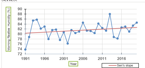
Fig. 7. Showing the trend and sen's slope of morning relative humidity for Akola district. It indicates that Man-Kendall test has p- value greater than level of significance. i.e. 0.05, so as per test statistics it is concluded that morning relative humidity does not have trend in it's time series.
