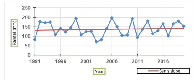
Fig. 4. Showing the trend and sen's slope of rainfall for Akola district. It indicates that Man-Kendall test has p-value greater than level of significance. i.e. 0.05, so as per test statistics it is concluded that rainfall does not have trend in it's time series.
